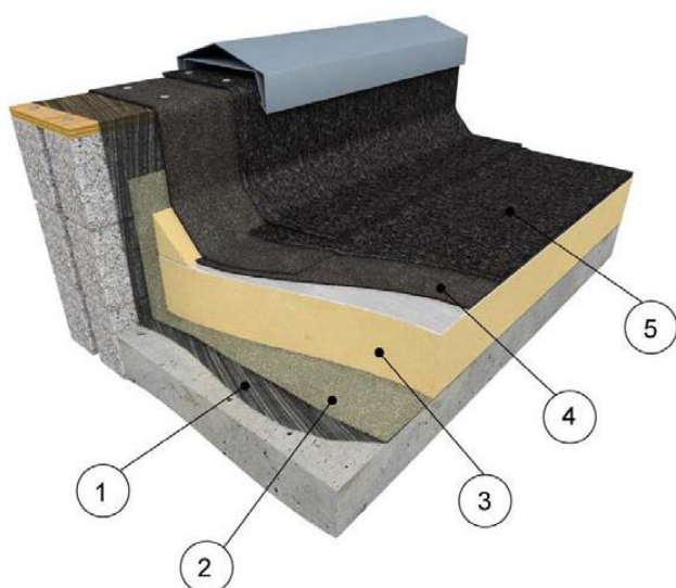
Figure 3 - Parapet detail
