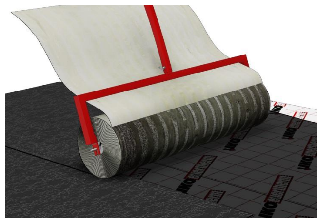
Figure 2 – application of IKO Ultra T-F Underlay
